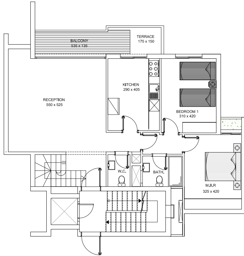
LOWER LEVEL
